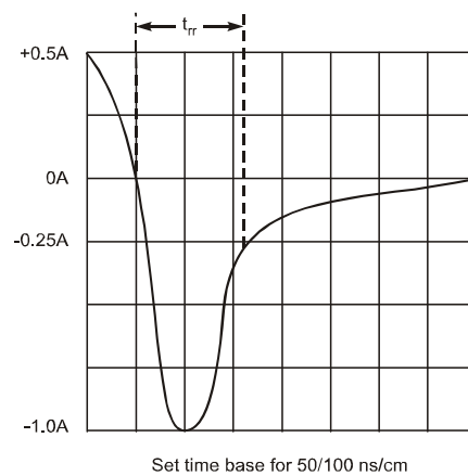
Fig. 5 Reverse Recovery Time Characteristic and Test Circuit
