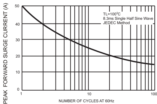
Fig. 3 Forward Surge Current Derating Curve
