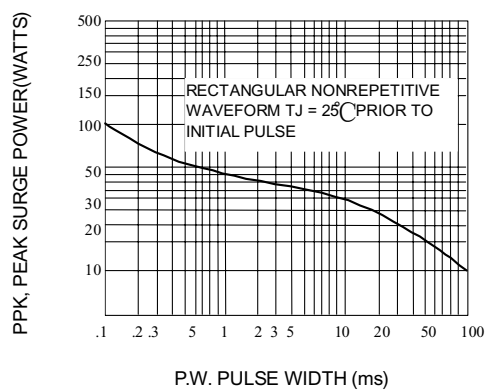
Fig. 2-MAXIMUM SURGE POWER
