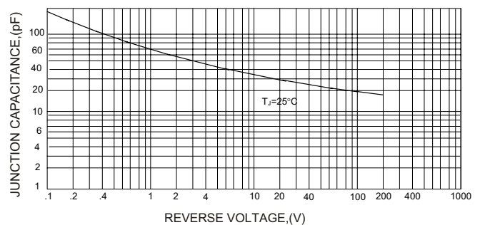
Fig. 6 Typical Junction Capacitance
