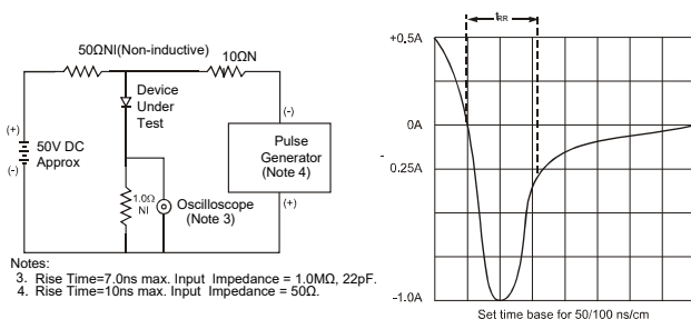
Fig. 5 Reverse Recovery Time Characteristic and Test Circuit
