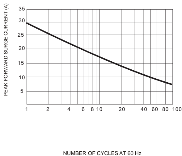
Fig. 3 Surge Current Derating Curve
