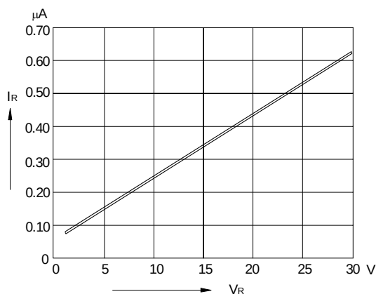
FIG.2-REVERSE CURRENT VERSUS CONTINUOUS REVERSE VOLTAGE
