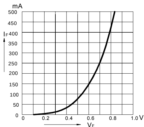
FIG.1-FORWARD CURRENT VERSUS FORWARD VOLTAGE (TYPICAL VALUES)
