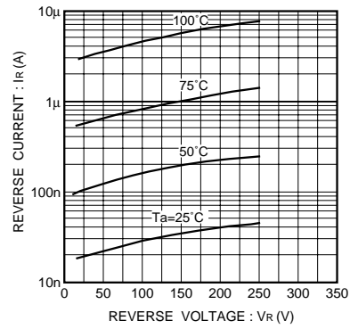
Fig.2 Reverse characteristics
