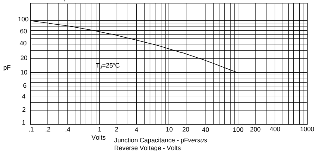
Figure 3 Junction Capacitance
