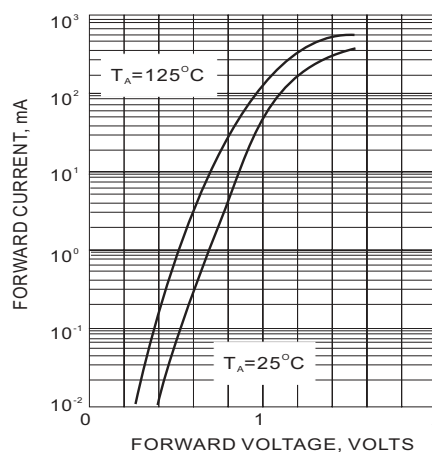
Fig.3 FORWARD CHARACTERISTICS
